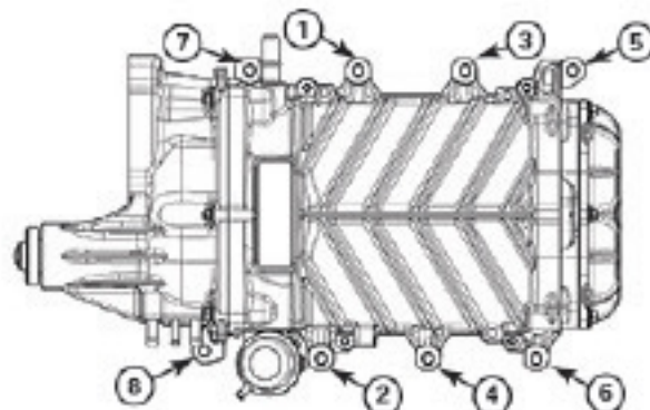
Supercharger bolt tightening sequence
